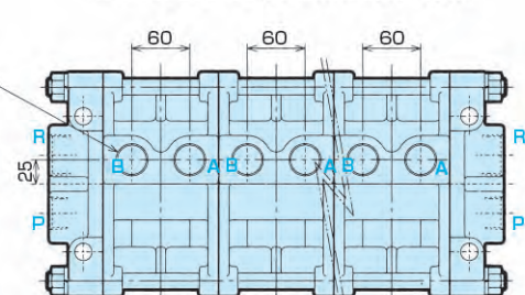
MVM5F-08-SP2 type (Lower piping type)
